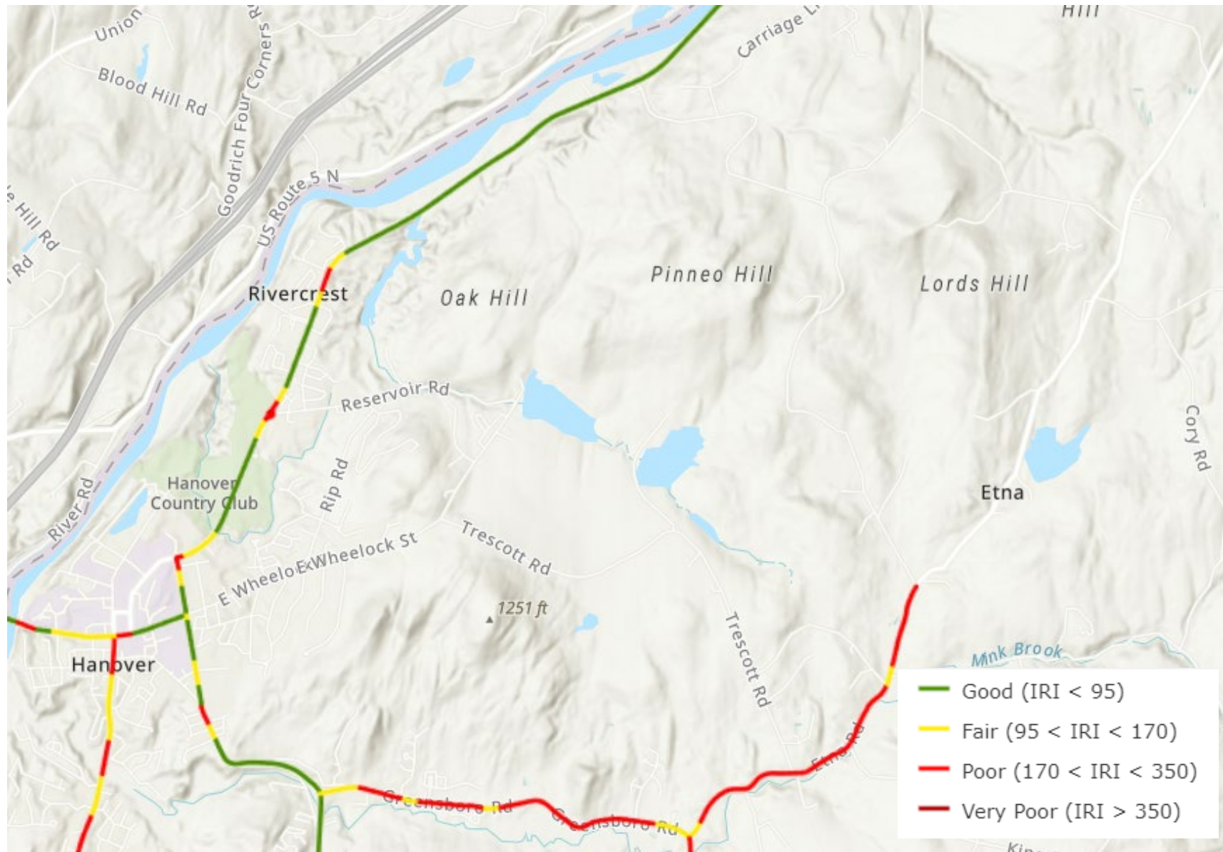
Figure E-5: Pavement Condition of NHDOT Inventoried Roads (2022)
